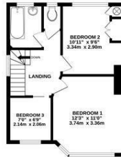
1ST FLOOR 390 sq ft (36.3 sq m.) approx.
